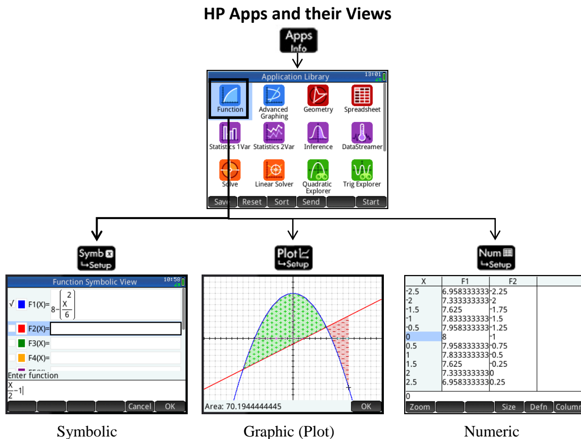
Figure 1. HP Prime apps and their views
